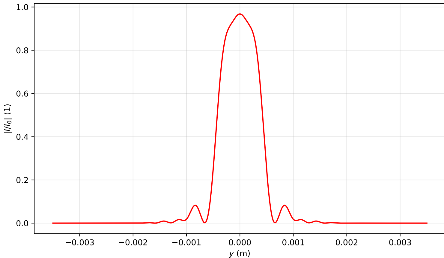
Intensity profile I(x=0, y, z=1.672)/I_0 , P_{in}=2.0P_{cr} , artificial time
